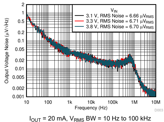
图 5-66. Noise vs Frequency and V_{IN}
