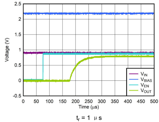
图 6-16. Start-Up With V_{\text{IN}} and V_{\text{BIAS}} Before V_{\text{EN}}
