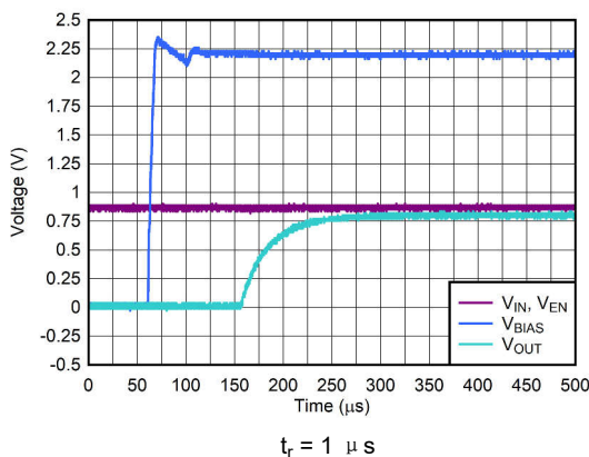
图 6-17. Start-Up With V_{\text{IN}} and V_{\text{EN}} Before V_{\text{BIAS}}
