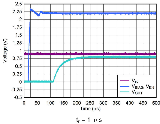
图 6-15. Start-Up With V_{\text{IN}} Before V_{\text{BIAS}} and V_{\text{EN}}
