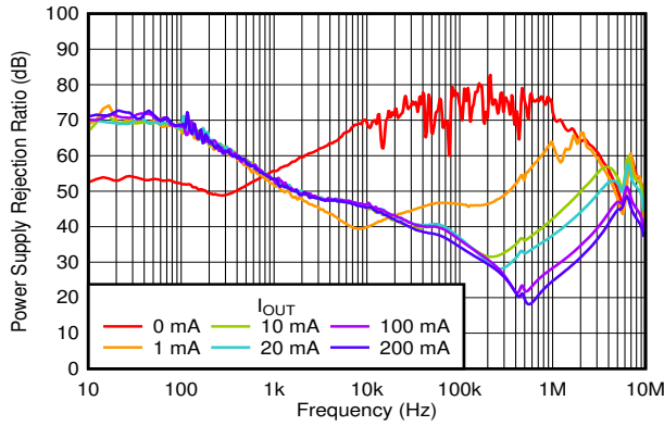
V_{IN} = 2.8\text{ V} , V_{OUT} = 1.8\text{ V} , C_{OUT} = 1\text{ }\mu\text{F} 图 6-43. PSRR vs Frequency and I_{OUT}
