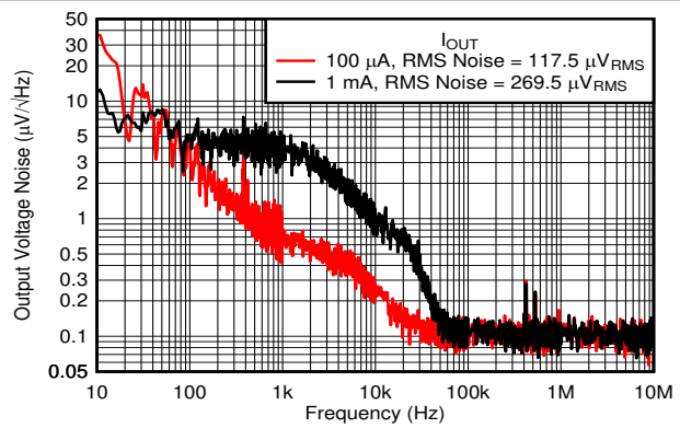
V_{OUT} = 1.8\text{ V} , V_{IN} = 2.8\text{ V} , C_{OUT} = 1\text{ }\mu\text{F} 图 6-48. Output Noise vs Frequency and I_{OUT}
