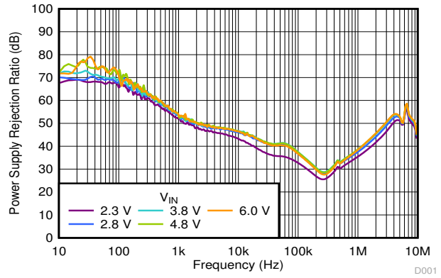
V_{OUT} = 1.8\text{ V} , I_{OUT} = 20\text{ mA} , C_{OUT} = 1\text{ }\mu\text{F} 图 6-44. PSRR vs Frequency and V_{IN}
