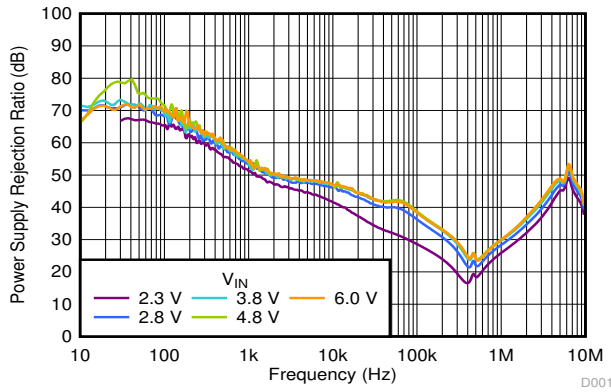
V_{OUT} = 1.8\text{ V} , I_{OUT} = 100\text{ mA} , C_{OUT} = 1\text{ }\mu\text{F} 图 6-45. PSRR vs Frequency and V_{IN}
