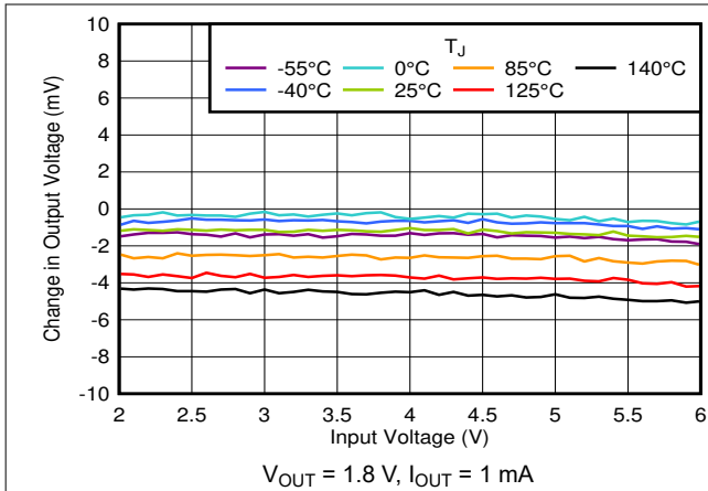
图 6-25. Line Regulation vs V_{IN} and Temperature
