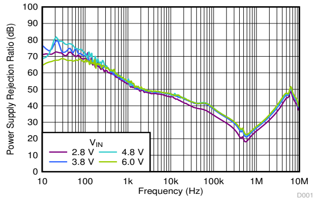
V_{OUT} = 1.8\text{ V} , I_{OUT} = 200\text{ mA} , C_{OUT} = 1\text{ }\mu\text{F} 图 6-46. PSRR vs Frequency and V_{IN}
