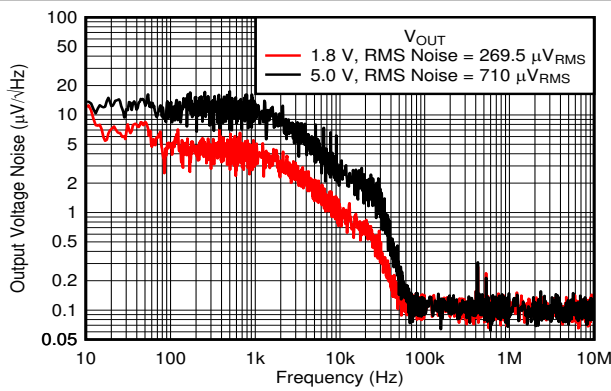
V_{IN} = V_{OUT} + 1.0\text{ V} , I_{OUT} = 1\text{ mA} , C_{OUT} = 1\text{ }\mu\text{F} 图 6-47. Output Noise vs Frequency and V_{OUT}
