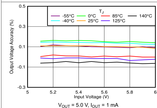
图 6-29. Output Accuracy vs V_{IN} and Temperature
