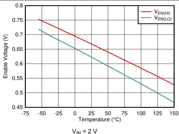
图 6-12. V_{EN(HI)} and V_{EV(LO)} Threshold vs Temperature
