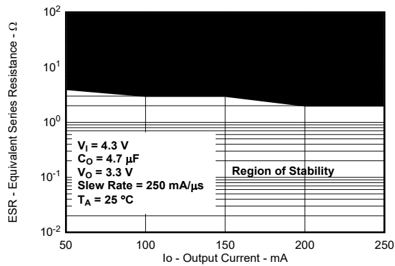
图 5-47. Typical Region of Stability ESR vs Output Current (Legacy Chip)
