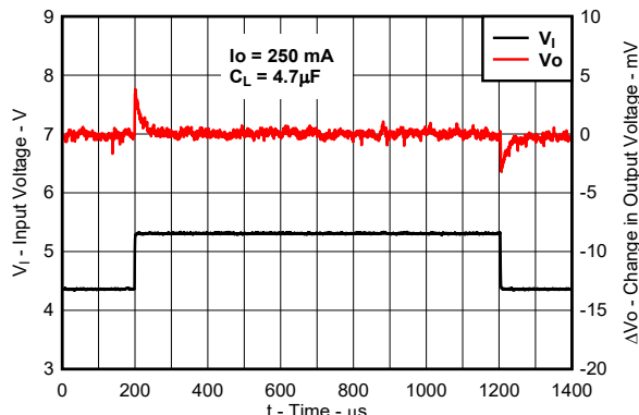
图 7-5. TPS76633 Line Transient Response (New Chip)
