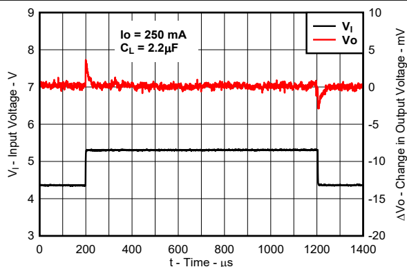
图 7-4. TPS76633 Line Transient Response (Legacy Chip)
