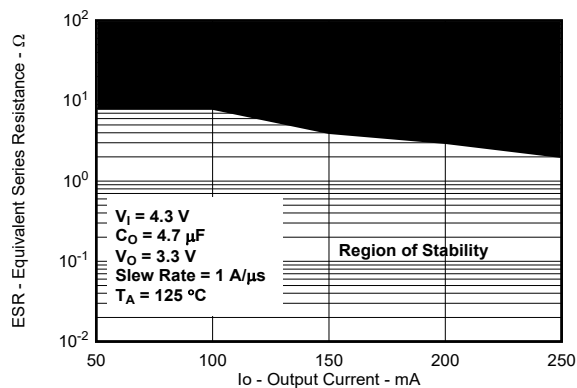
图 5-49. Typical Region of Stability ESR vs Output Current (New Chip)
