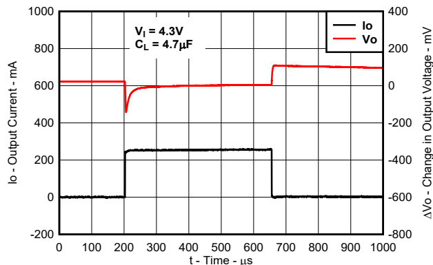
图 5-39. TPS76633 Load Transient Response (New Chip)
