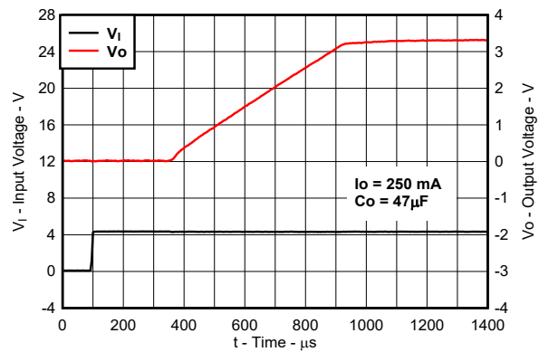
图 5-45. TPS76633 Output Voltage vs Time (New Chip)
