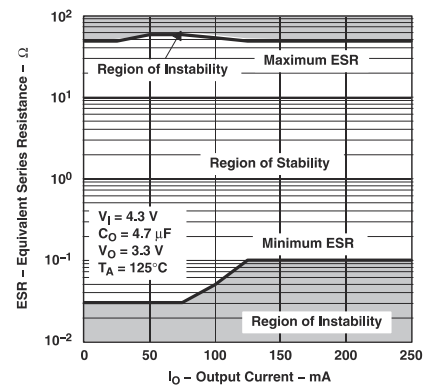
图 5-48. Typical Region of Stability ESR vs Output Current (New Chip)
