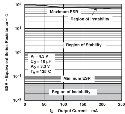
图 5-54. Typical Region of Stability ESR vs Output Current (New Chip)
