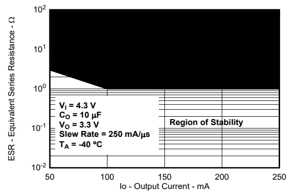
图 5-60. Typical Region of Stability ESR vs Output Current (Legacy Chip)
