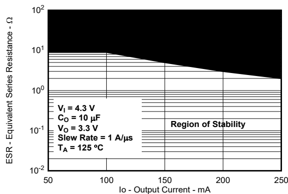
图 5-55. Typical Region of Stability ESR vs Output Current (New Chip)
