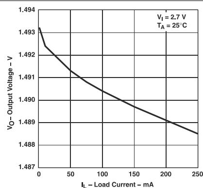
图 5-3. TPS76633 Output Voltage vs Load Current (New Chip)
