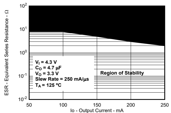
图 5-50. Typical Region of Stability ESR vs Output Current (Legacy Chip)
