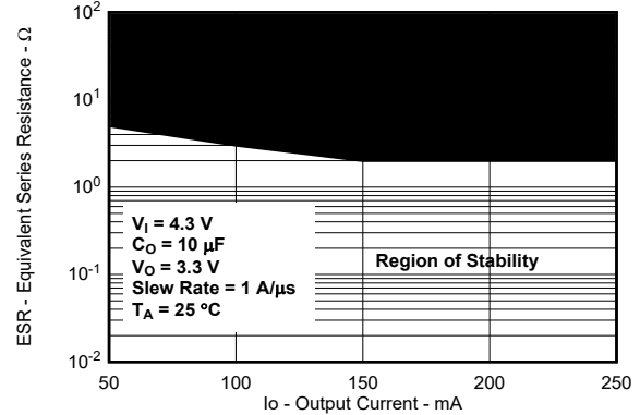
图 5-54. Typical Region of Stability ESR vs Output Current (New Chip)
