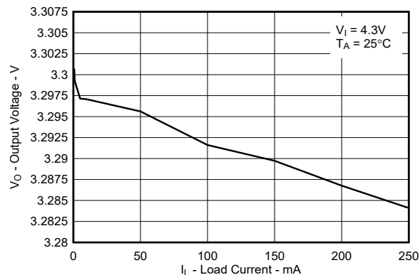
图 5-3. TPS76633 Output Voltage vs Load Current (New Chip)
