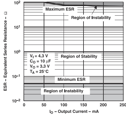
图 5-53. Typical Region of Stability ESR vs Output Current (Legacy Chip)
