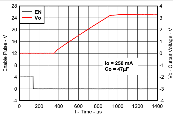
图 5-41. TPS76633 Output Voltage vs Time (Legacy Chip)
