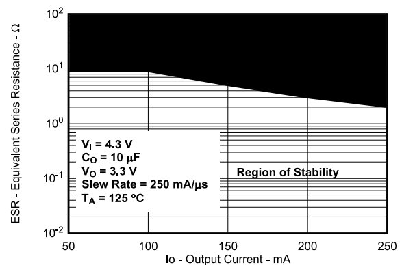
图 5-56. Typical Region of Stability ESR vs Output Current (Legacy Chip)
