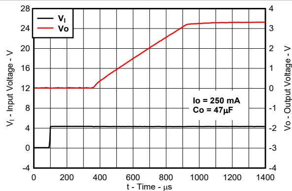
图 7-12. TPS76633 Output Voltage vs Time (New Chip)
