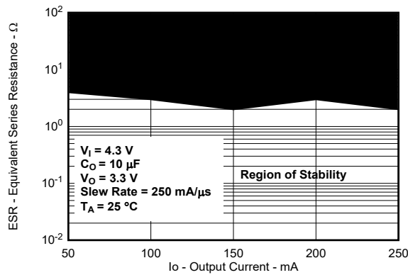
图 5-53. Typical Region of Stability ESR vs Output Current (Legacy Chip)
