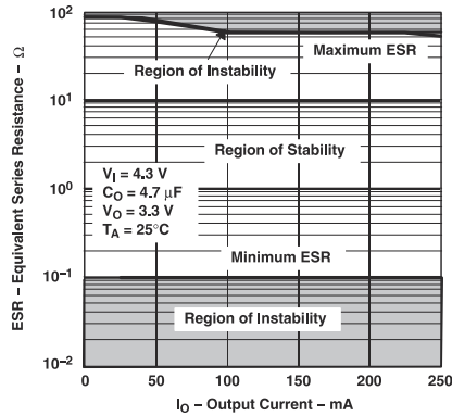
图 5-47. Typical Region of Stability ESR vs Output Current (Legacy Chip)
