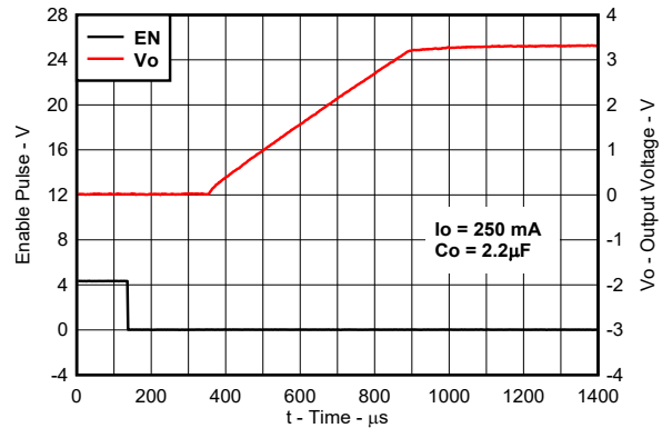
图 7-11. TPS76633 Output Voltage vs Time (New Chip)
