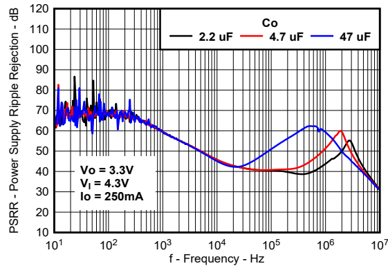
图 5-26. TPS76633 Power-Supply Ripple Rejection vs Frequency and Output Capacitor (New Chip)
