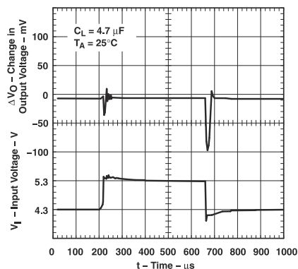
图 7-4. TPS76633 Line Transient Response (Legacy Chip)
