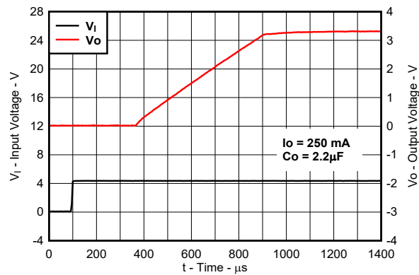
图 5-44. TPS76633 Output Voltage vs Time (New Chip)
