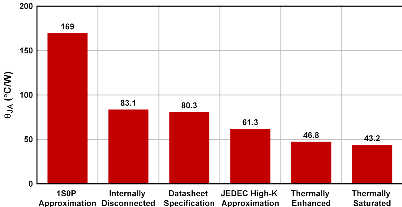
Figure 7-8. TPS746-Q1 (WSON) R_{\theta JA} vs Board Layout
