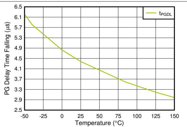
Figure 5-20. t_{PGDL} vs Temperature
