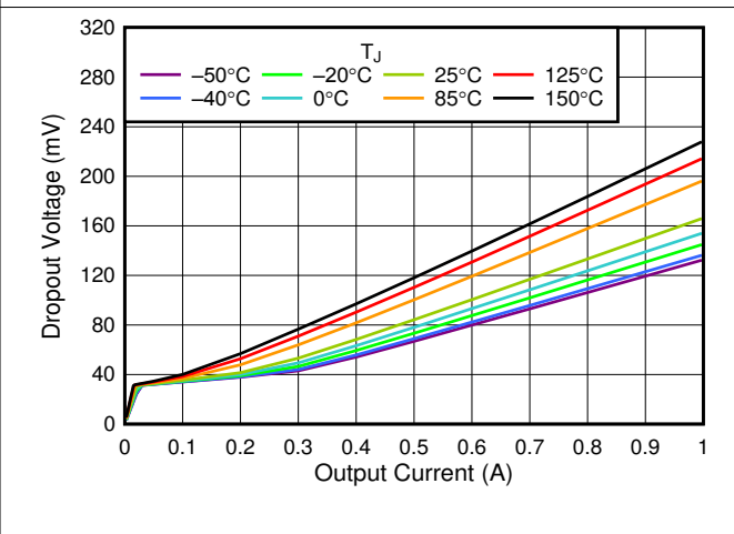
Figure 5-4. 3.3-V Dropout Voltage vs I_{OUT}
