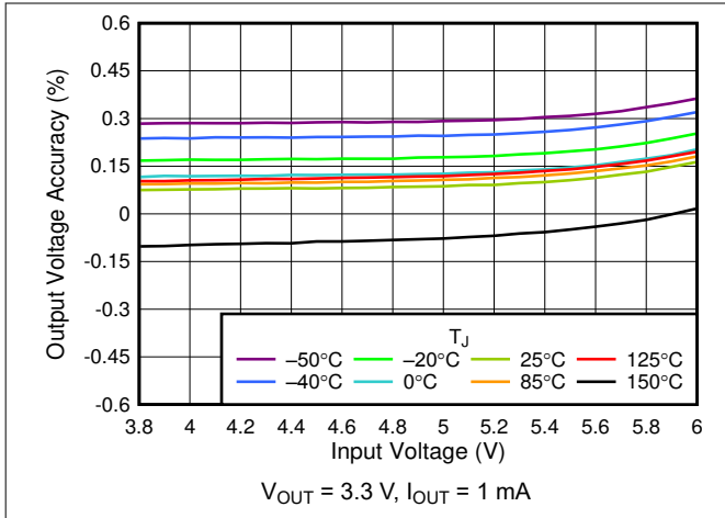
Figure 5-1. 3.3-V Line Regulation vs V_{IN}
