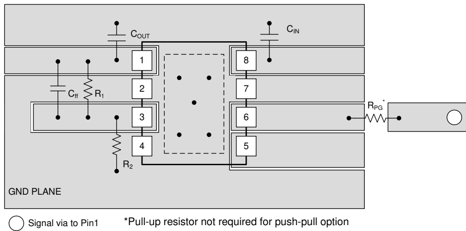
Figure 7-12. Layout Example for the DRB package
