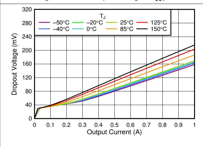
Figure 5-6. 5.5-V Dropout Voltage vs I_{OUT}
