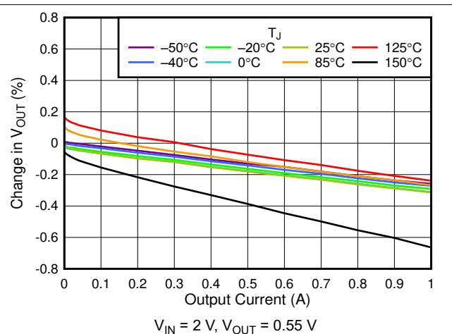
Figure 5-12. 0.55-V Load Regulation vs I_{OUT}
