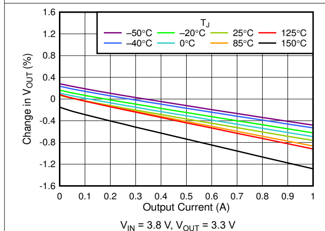
Figure 5-11. 3.3-V Load Regulation vs I_{OUT}
