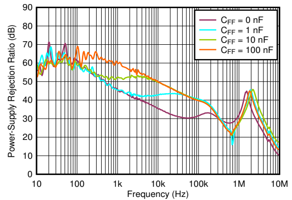
Figure 5-38. PSRR vs Frequency and C_{FF}
