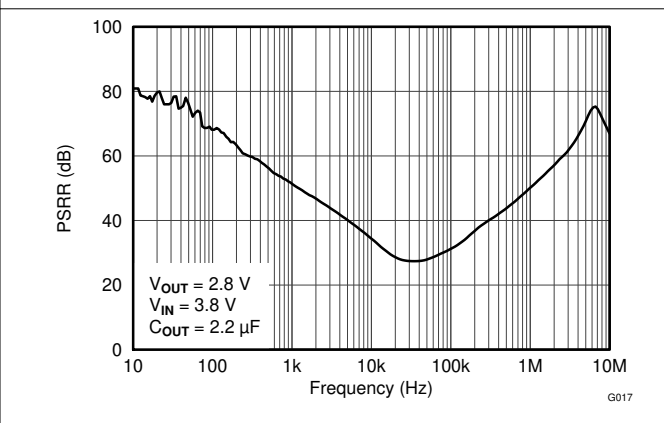
图 6-18. Power-Supply Rejection Ratio vs Frequency
