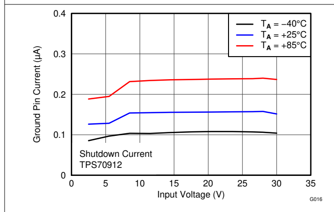
图 6-17. Shutdown Current vs V_{IN} and Temperature
