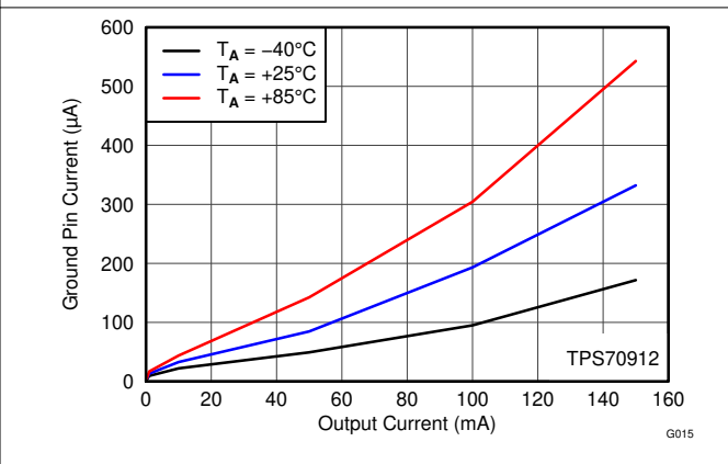
图 6-16. GND Current vs I_{OUT} and Temperature
