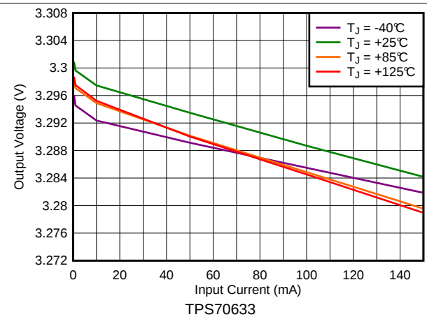
Figure 4. 3.3-V Load Regulation vs I_{OUT} and Temperature
