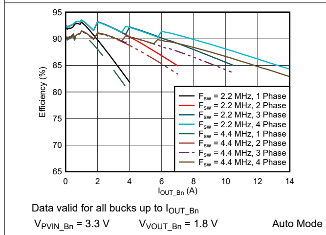
图 9-6. BUCK Efficiency in Varied Phase Configuration, 3.3 V Input
