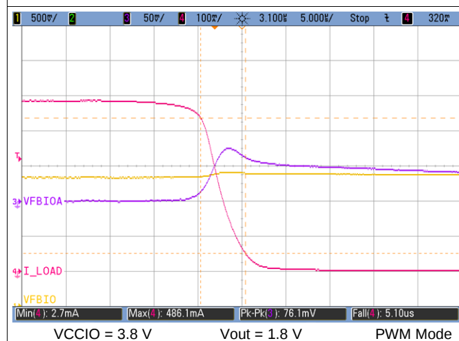
图 7-6. VDDIO Falling Load Transient Response
