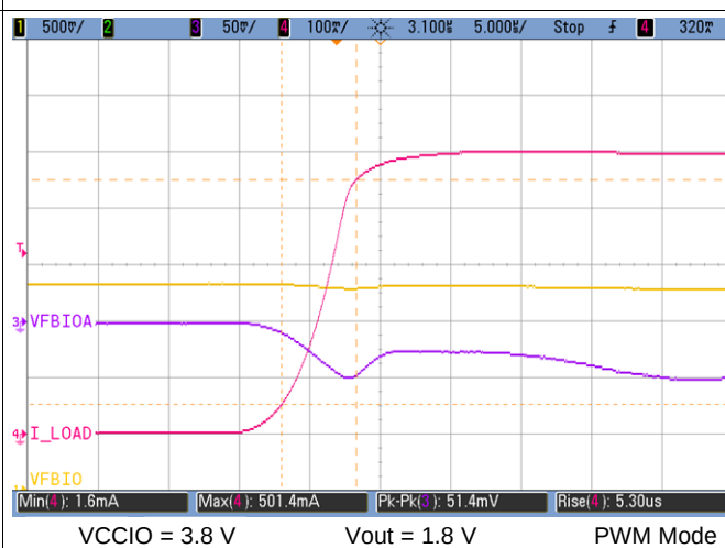
图 7-7. VDDIO Rising Load Transient Response
