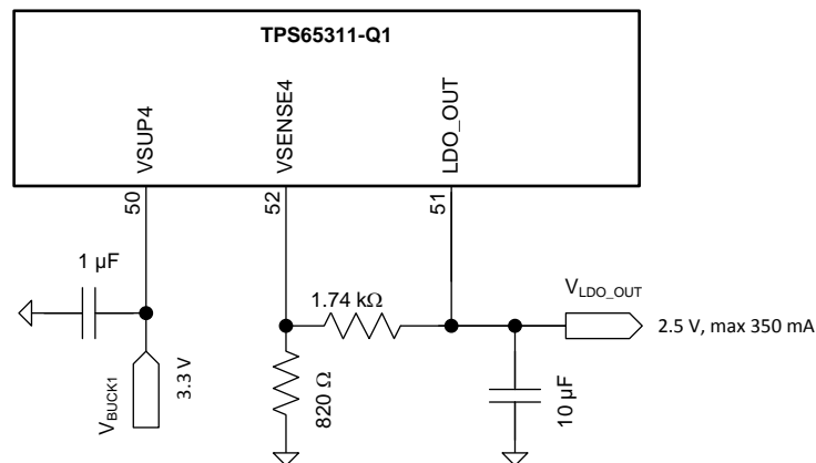
Figure 38. Linear Regulator Schematic
