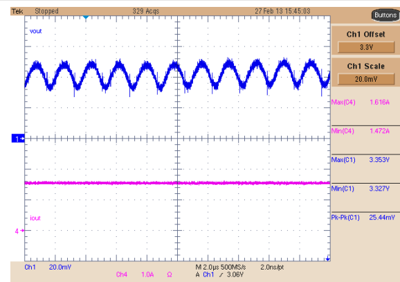
图 8-46. Buck 3 Ripple, 3-A Load
