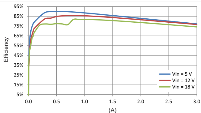
图 6-2. Efficiency, LOW_P Mode
