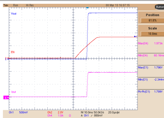
图 8-24. Buck 2 Start-Up, 2-A Load
