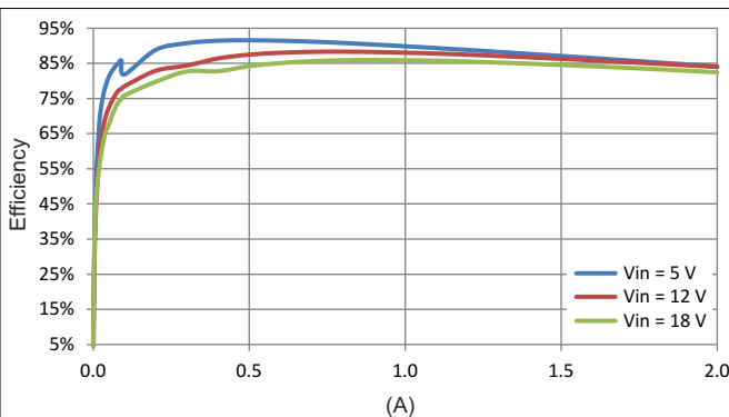
图 6-8. Efficiency, LOW_P Mode
