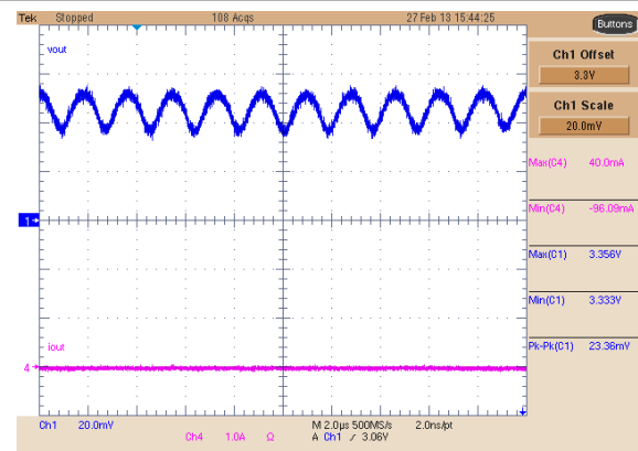
图 8-44. Buck 3 Ripple, No Load
