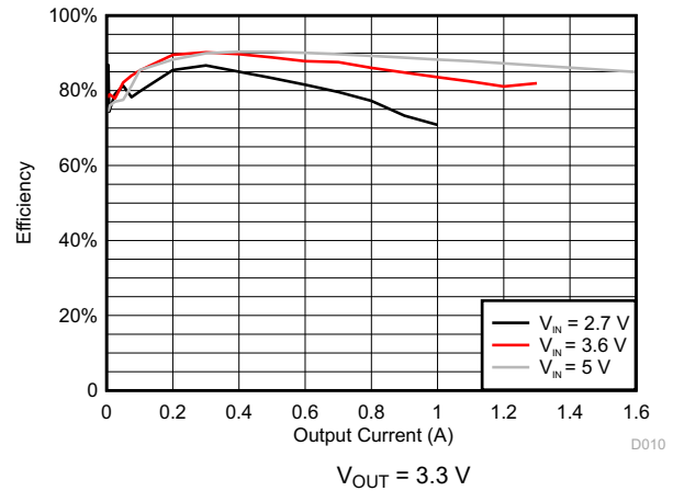
Figure 8-5. DCDC4 Efficiency
