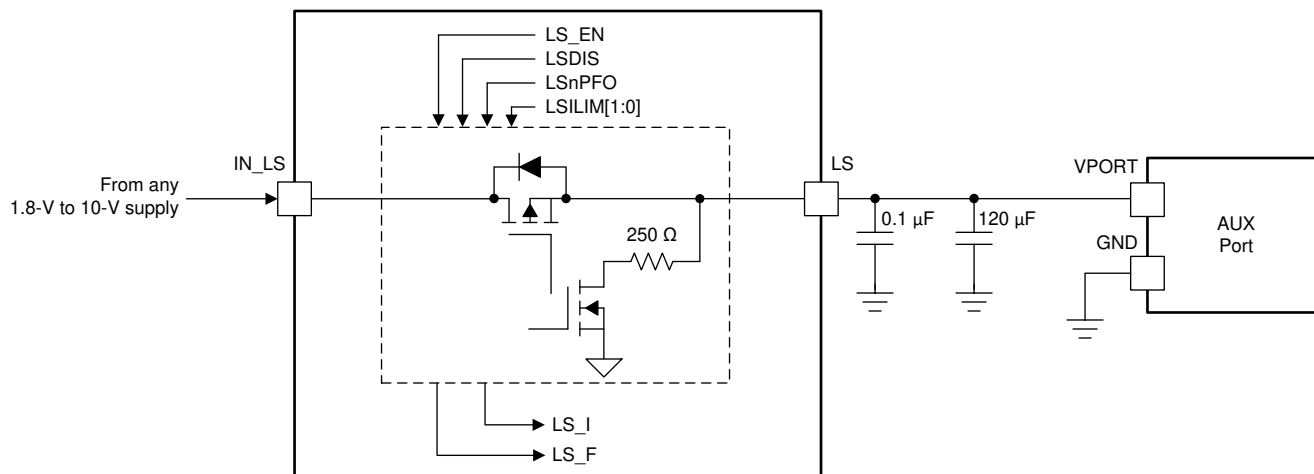
Figure 6-10. Typical Application of Load Switch
