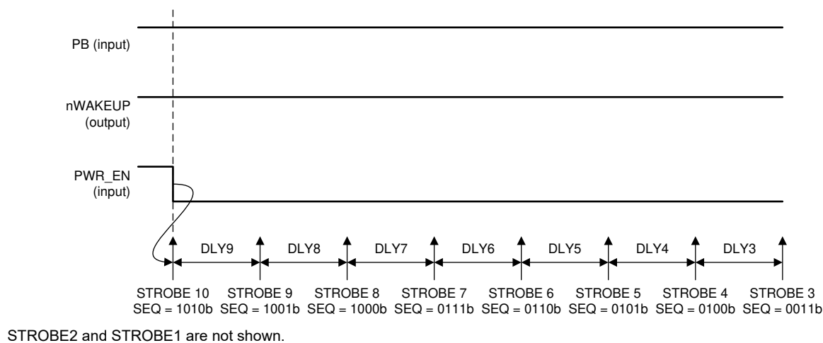
Figure 6-5. Power-Down Sequences to SUSPEND State; PWR_EN is Power-Down Event
