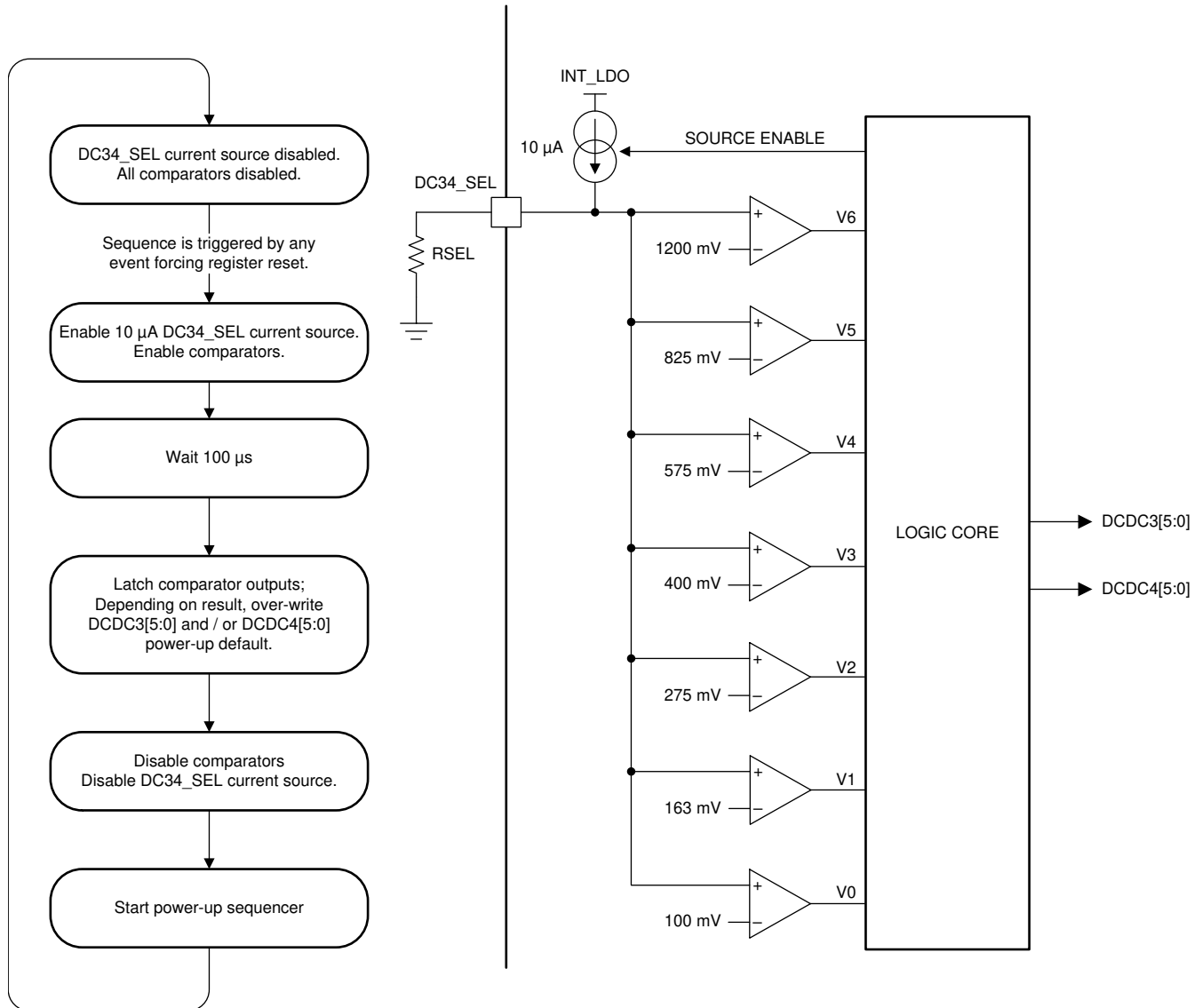
Figure 6-13. Left: Flow Chart for Selecting DCDC Power-Up Default Voltage Right: Comparator Circuit
