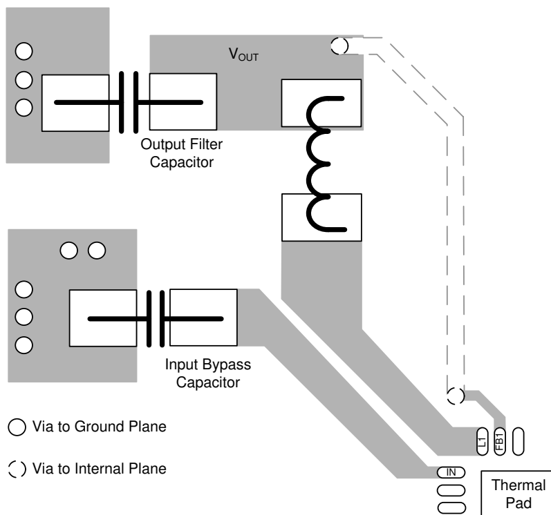
Figure 8-6. Layout Recommendation
