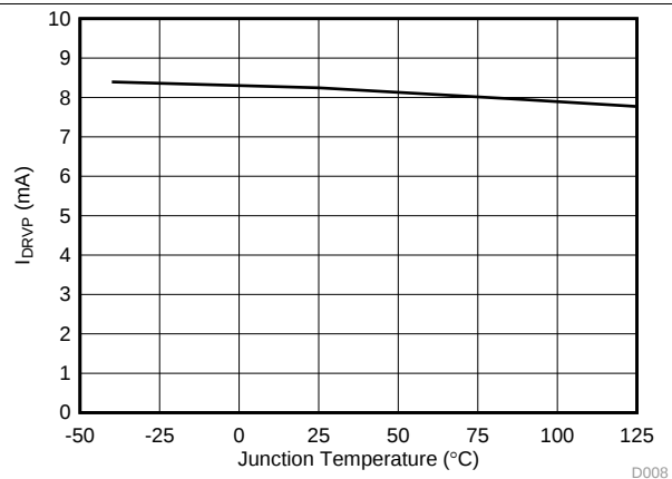
Figure 8. V_{(GH)} charge-pump DRVP drive current
