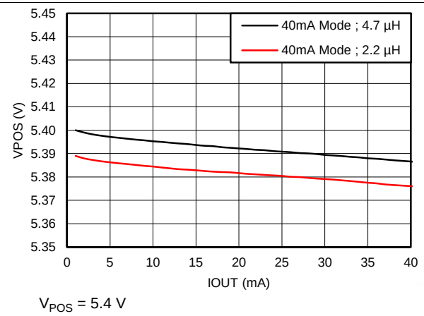
Figure 44. Load Regulation
