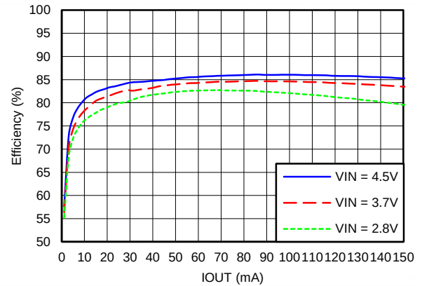
Figure 84. Combined Efficiency — \pm 5.4\text{ V} — SYNC = HIGH L = 2.2\text{ }\mu\text{H}
