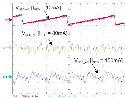
Figure 86. V_{\text{NEG}} Output Voltage Ripple — SYNC = HIGH — L = 2.2\text{ }\mu\text{H} — C_{\text{OUT}} = 10\text{ }\mu\text{F}
