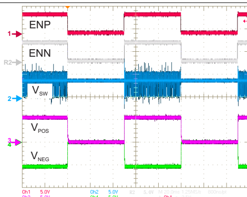
Figure 67. Power-Up/Down With Active Discharge
