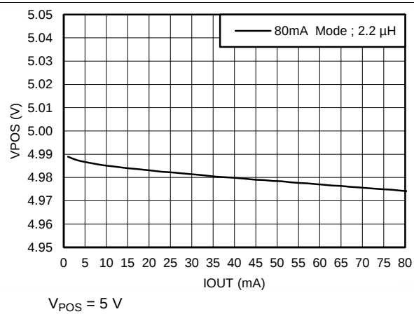
Figure 73. Load Regulation
