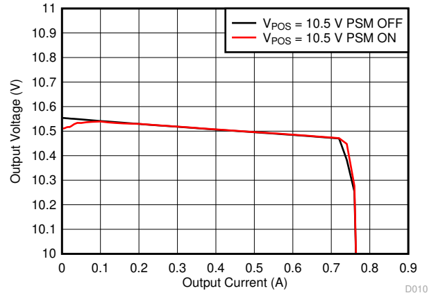
图 8-7. Boost Converter ( V_{POS} ) Output Voltage vs Output Current
