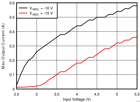
图 6-2. Inverting Converter ( V_{\text{POS}} ) Output Current vs Input Voltage
