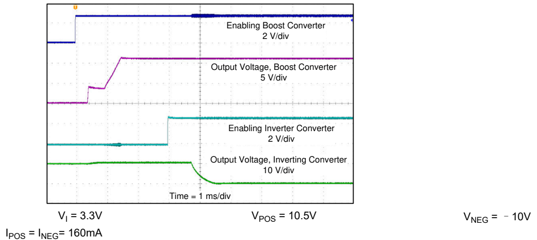
图 8-20. Boost and Inverting Converter Start-Up Into Load
