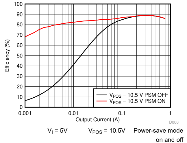
图 8-3. Boost Converter ( V_{POS} ) Efficiency vs Output Current
