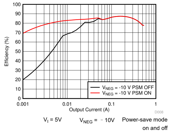
图 8-5. Inverting Converter ( V_{NEG} ) Efficiency vs Output Current
