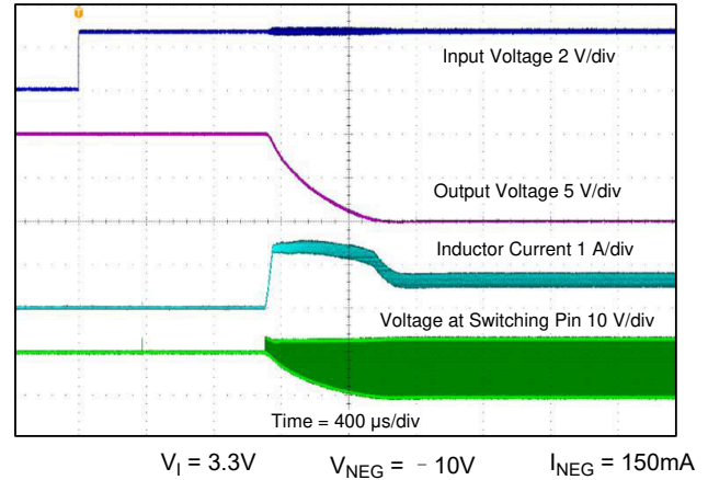
图 8-19. Inverting Converter ( V_{NEG} ) Start-Up Into Load
