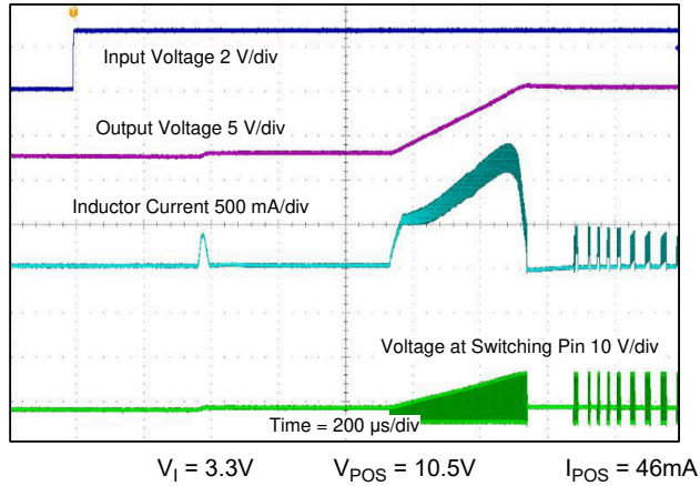
图 8-18. Boost Converter ( V_{POS} ) Start-Up Into Load
