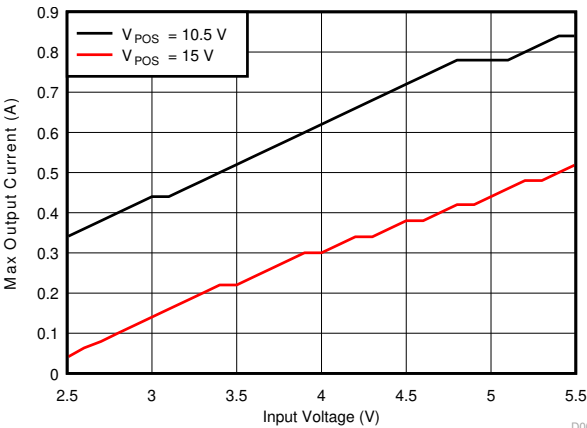
图 6-1. Boost Converter ( V_{\text{POS}} ) Maximum Output Current vs Input Voltage
