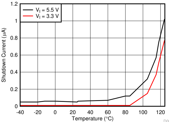
图 6-3. Shutdown Current (Into VIN and INN) Over Input Voltage
