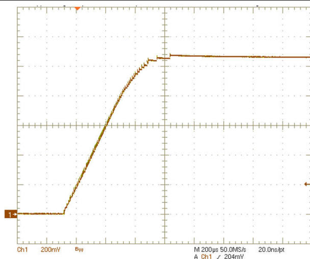
图 8-6. BUCK2 Controller Start-Up
