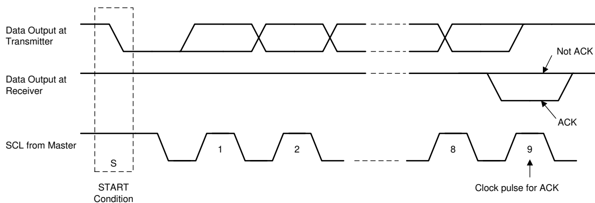
图 7-15. Acknowledge on the I 2 C Bus
