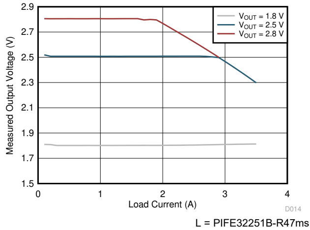
图 5-7. Converter Load Current Limitations with V_{IN} = 3.3V
