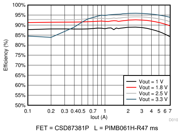
图 7-8. BUCK1 Efficiency at V_{IN} = 5 V in Auto Mode
