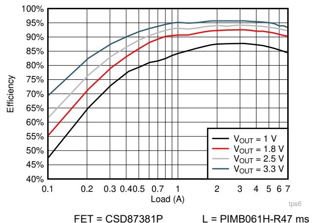
图 7-9. Example BUCK1 Efficiency at V_{IN} = 5 V in Forced PWM Mode
