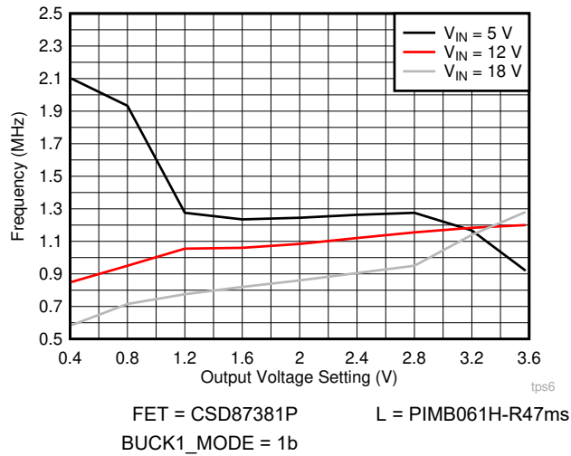
图 5-9. Controller Switching Frequency (Forced PWM Mode)
