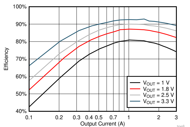
图 5-4. Example BUCK1 Efficiency at V_{IN} = 13V in Forced PWM Mode
