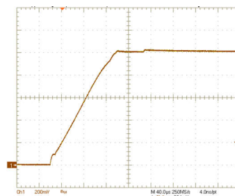
图 5-2. Example BUCK3 Converter Start-Up
