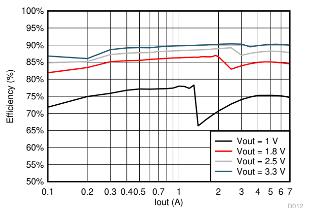
图 5-3. Example BUCK1 Efficiency at V_{IN} = 13V In Auto Mode
