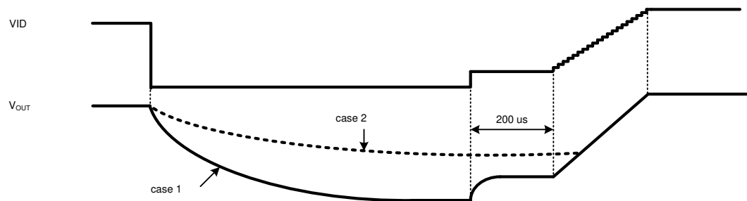
图 6-8. Decay Down to 0 V and Slew Up
