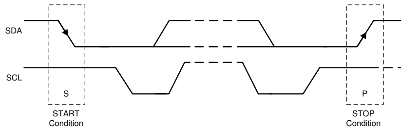
图 6-14. START and STOP Conditions
