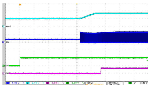
图 9-66. Start-Up Timing
