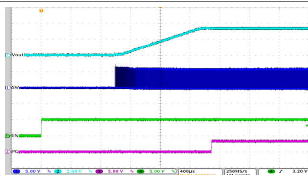
图 9-64. Start-Up Timing
