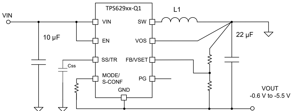
图 9-86. IBB Example with Adjustable Feedback
