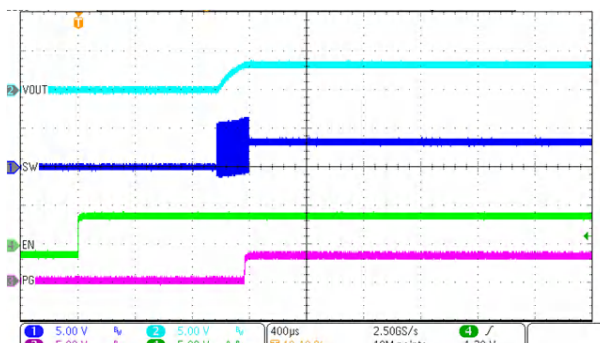
图 9-65. Start-Up Timing
