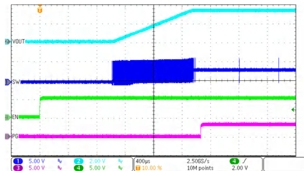
图 9-64. Start-Up Timing
