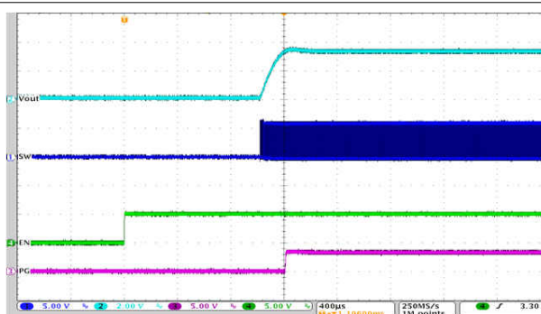
图 9-65. Start-Up Timing
