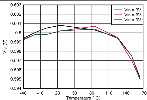
图 7-3. Feedback Voltage Accuracy - External Feedback Selected
