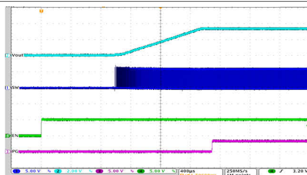
图 9-64. Start-Up Timing
