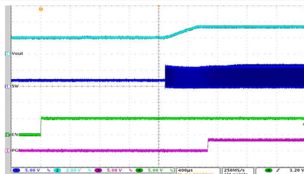
图 9-66. Start-Up Timing
