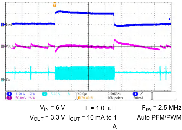
图 9-72. Load Transient Response
