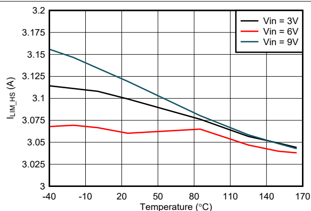
图 7-15. High Side I_{LIM} vs Temperature
