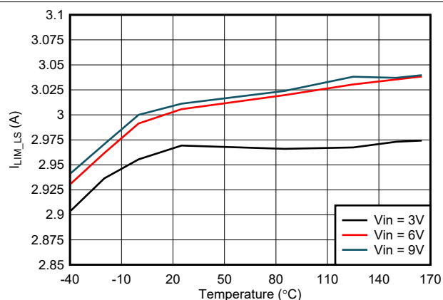
图 7-16. Low Side I_{LIM} vs Temperature
