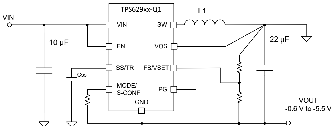
图 9-85. IBB Example with Adjustable Feedback
