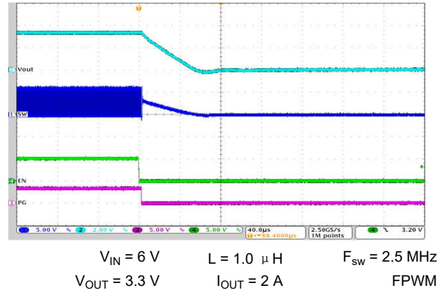
图 9-71. Shutdown Timing with Output Discharge Disabled
