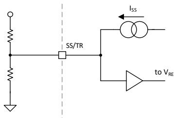
图 8-4. Tracking Operation Simplified Schematic
