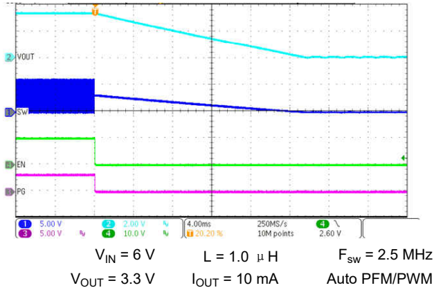
图 9-70. Shutdown Timing with Output Discharge Disabled
