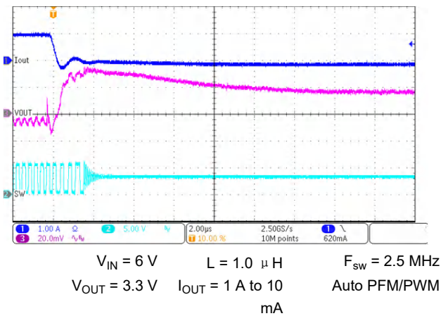
图 9-74. Load Transient Response Overshoot
