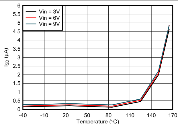
图 7-2. Shutdown Current vs Temperature
