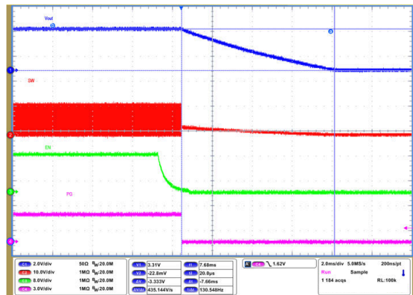
图 9-68. Shutdown Timing with Output Discharge Disabled
