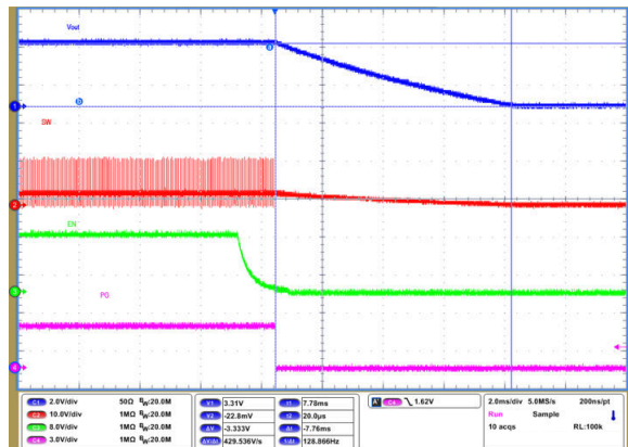
图 9-68. Shutdown Timing with Output Discharge Disabled
