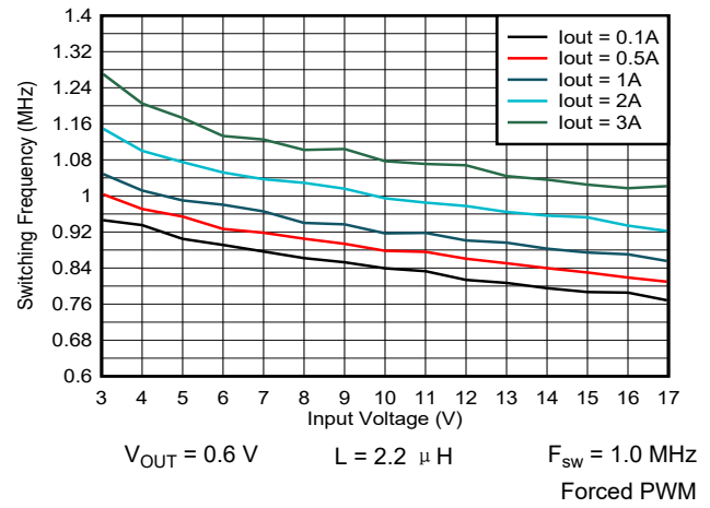
图 9-36. Switching Frequency vs Input Voltage
