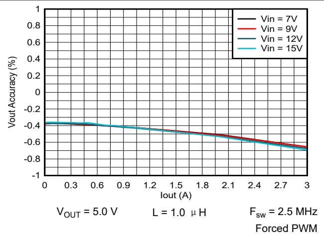
图 9-45. Output Voltage vs Output Current
