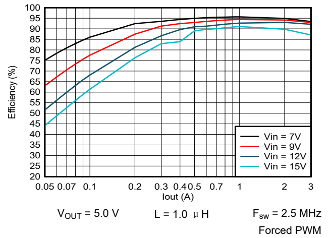
图 9-41. Efficiency vs Output Current
