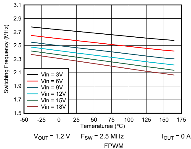
图 7-11. Switching Frequency vs Temperature
