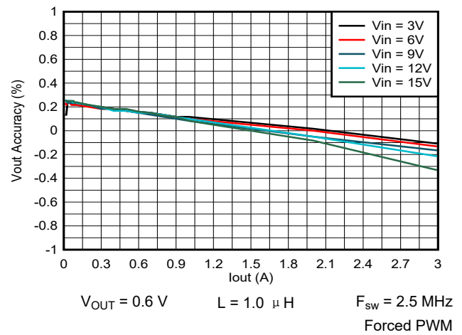
图 9-32. Output Voltage vs Output Current
