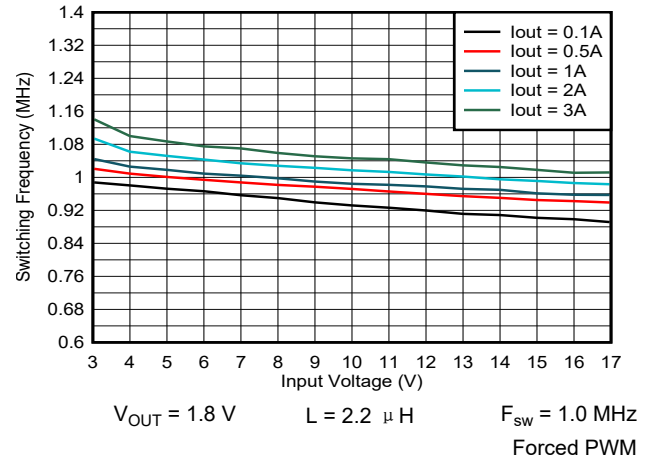
图 9-12. Switching Frequency vs Input Voltage
