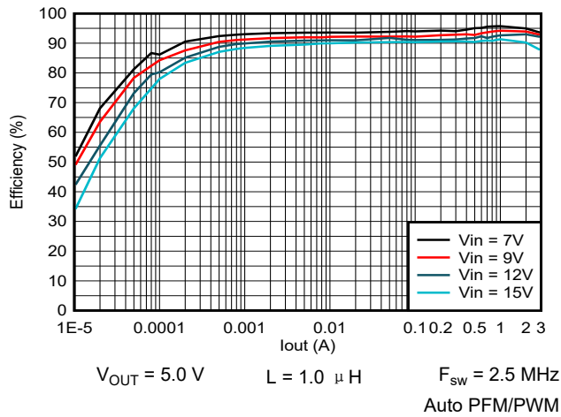
图 9-40. Efficiency vs Output Current
