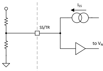
图 8-4. Tracking Operation Simplified Schematic
