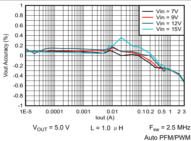
图 9-44. Output Voltage vs Output Current
