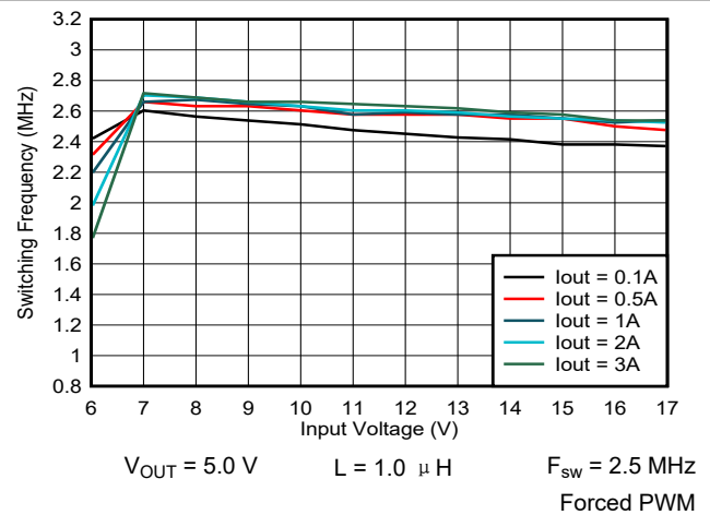
图 9-43. Switching Frequency vs Input Voltage
