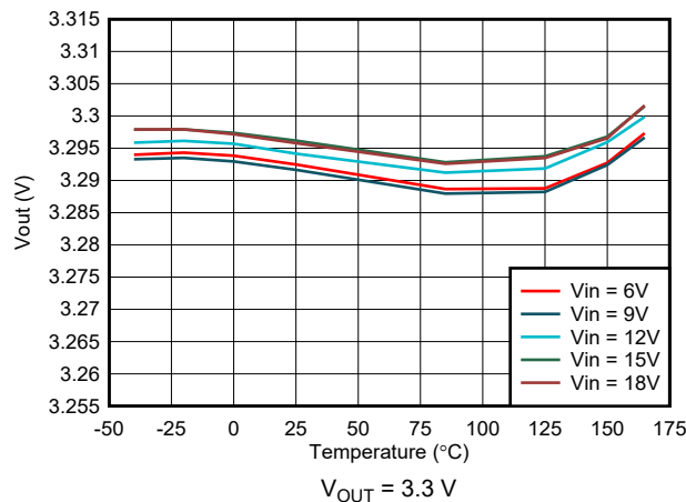
图 7-5. Output Voltage Accuracy - VSET Selected
