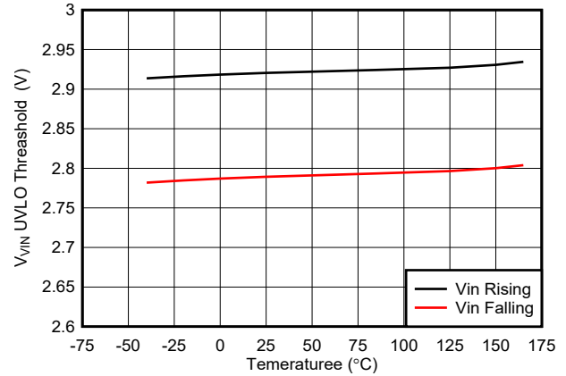
图 7-20. V_{VIN} UVLO Thresholds vs Temperature
