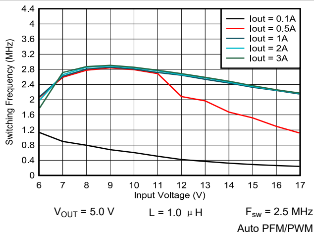
图 9-42. Switching Frequency vs Input Voltage
