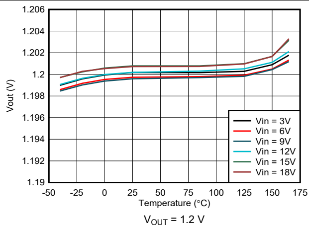
图 7-8. Output Voltage Accuracy - VSET Selected
