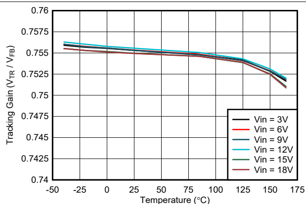
图 7-10. Tracking Voltage Gain vs Temperature
