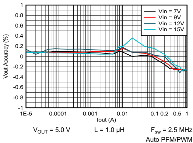
图 9-44. Output Voltage vs Output Current
