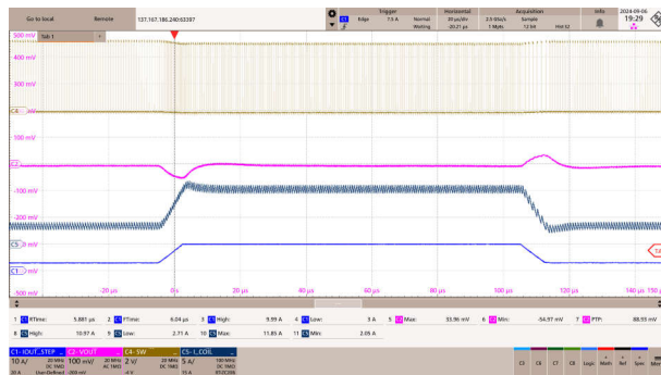
V_{IN} = 5.0V TPS6286A10 BOM = 4 \times 22 \mu F V_{OUT} = 0.9V I_{OUT} = 4A \text{ 至 } 10A
