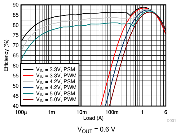
图 9-2. Efficiency
