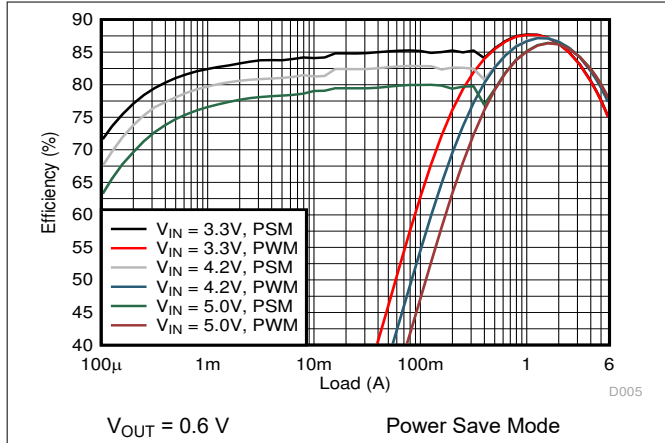
图 9-2. Efficiency
