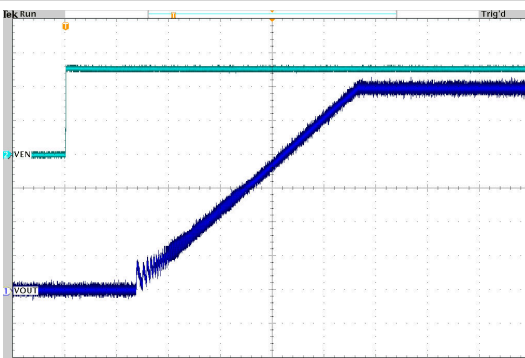
图 10-52. Start-Up Timing
