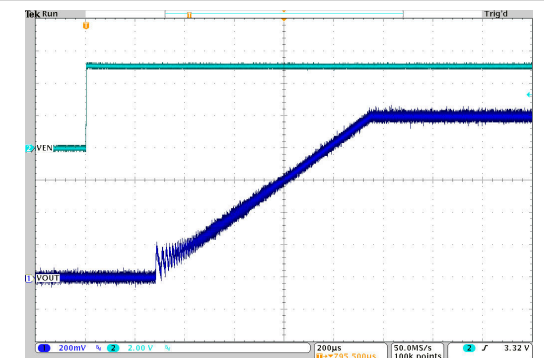
图 10-53. Start-Up Timing
