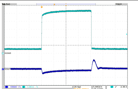
图 10-29. Load Transient Response
