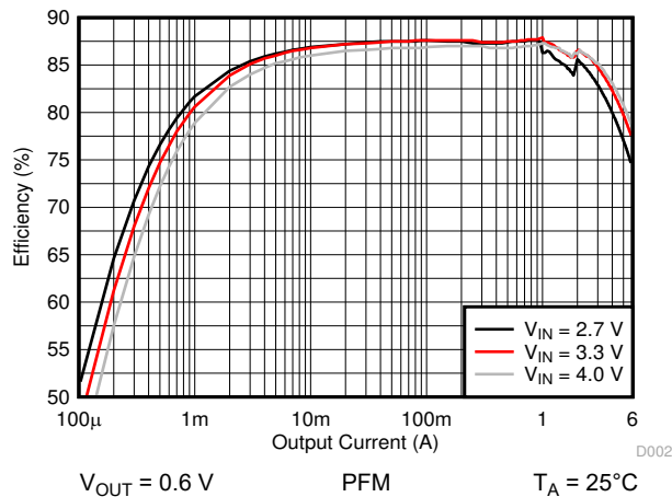
图 10-10. Efficiency Versus Output Current
