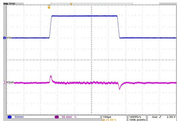
V_{OUT} = 3.3V PWM T_A = 25^\circ C I_{OUT} = 4A V_{IN} = 4.5V 至 5.5V 至 4.5V
