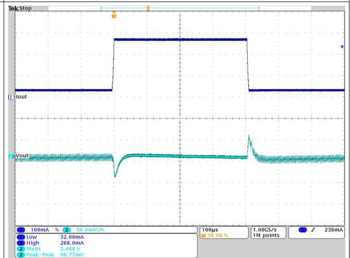
Figure 27. Load Transient Response; V_{OUT} = 2.5 V
