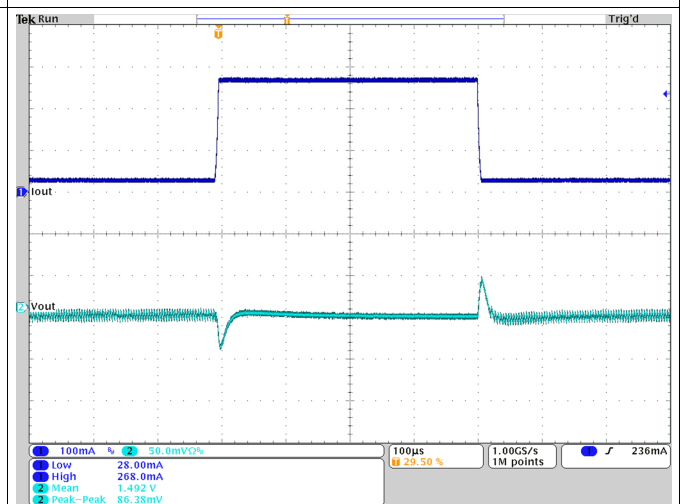
Figure 29. Load Transient Response; V_{OUT} = 1.5 V
