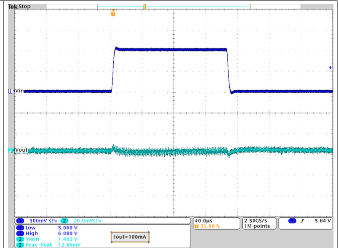
Figure 25. Line Transient Response; V_{OUT} = 1.5 V
