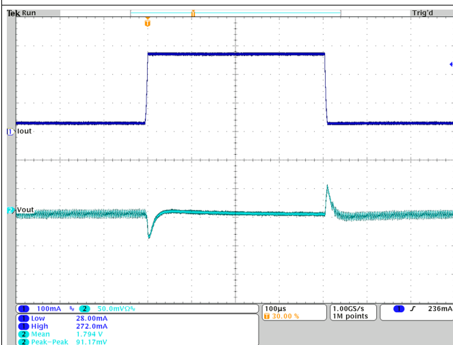
Figure 28. Load Transient Response; V_{OUT} = 1.8 V
