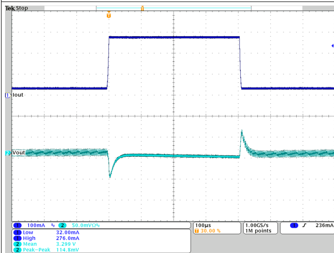
Figure 26. Load Transient Response; V_{OUT} = 3.3 V
