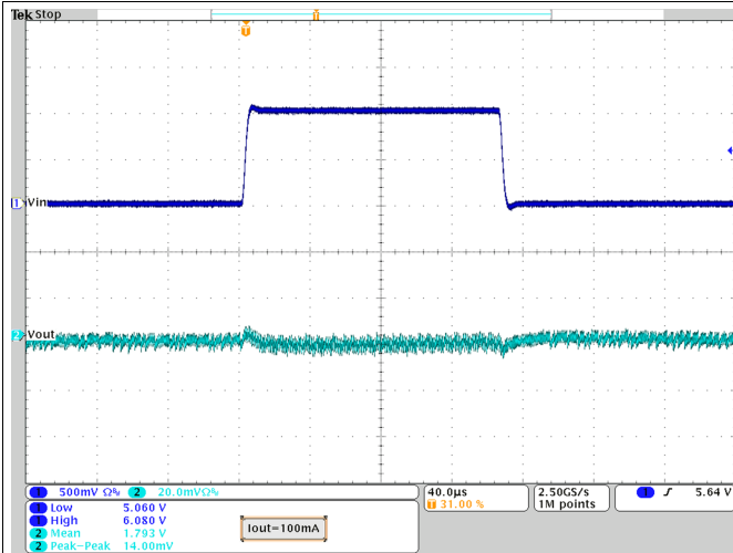
Figure 24. Line Transient Response; V_{OUT} = 1.8 V
