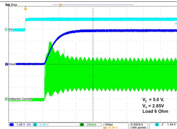
Figure 22. Start-Up
