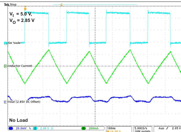
Figure 19. PWM Operation
