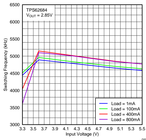
Figure 17. PWM Switching Frequency Vs Input Voltage
