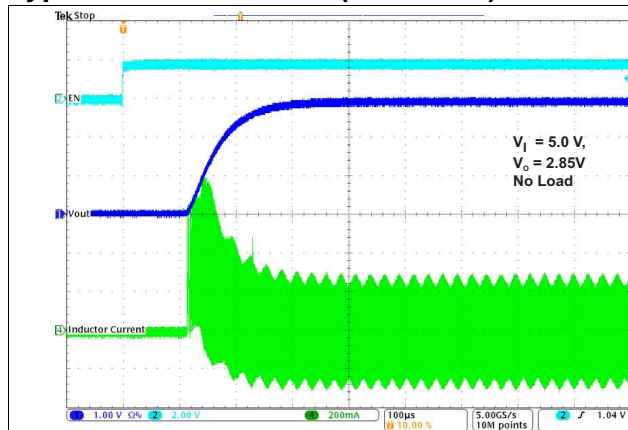
Figure 21. Start-Up
