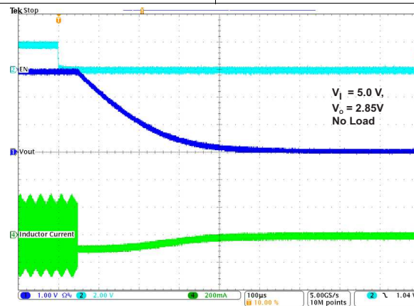
Figure 23. Shutdown
