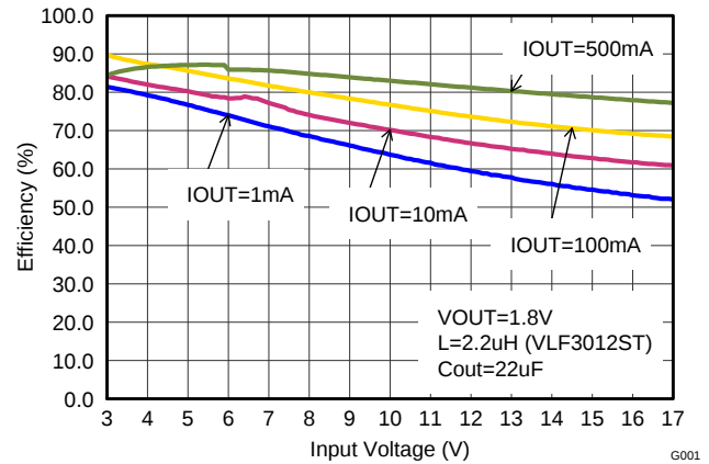
Figure 15. Efficiency vs Input Voltage, V_{OUT} = 1.8 V
