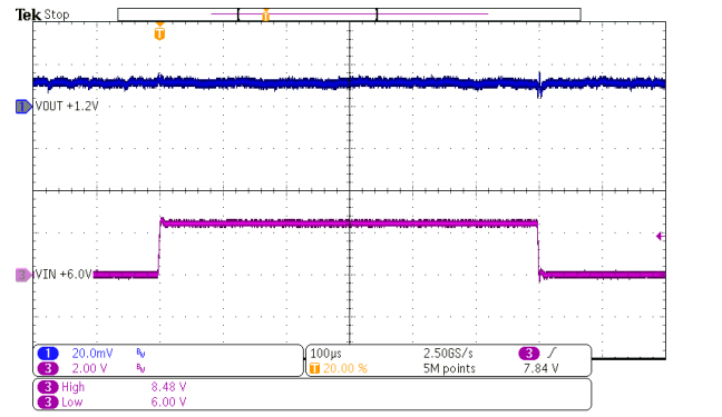
图 10-33. Line Transient Response
