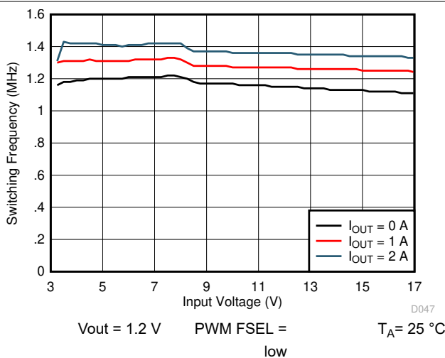
图 10-67. Switching Frequency vs Input Voltage
