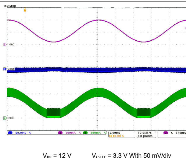
图 9-30. PWM-PSM-Transition
