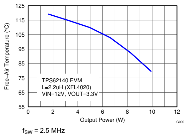
图 9-39. Maximum Ambient Temperature
