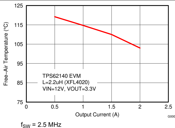
图 9-38. Maximum Ambient Temperature
