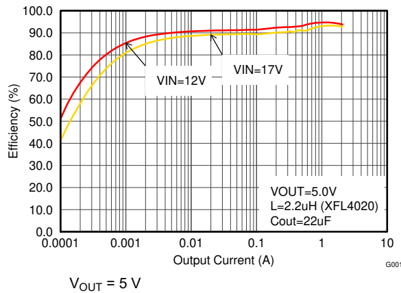
图 9-4. Efficiency With 1.25 MHz
