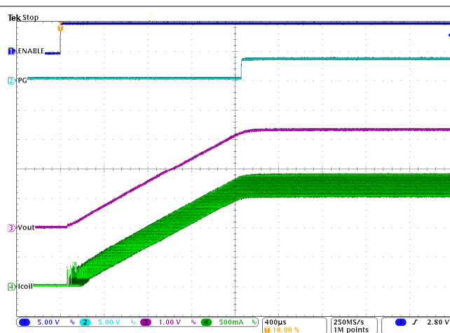
图 9-35. Start-Up into 2 A
