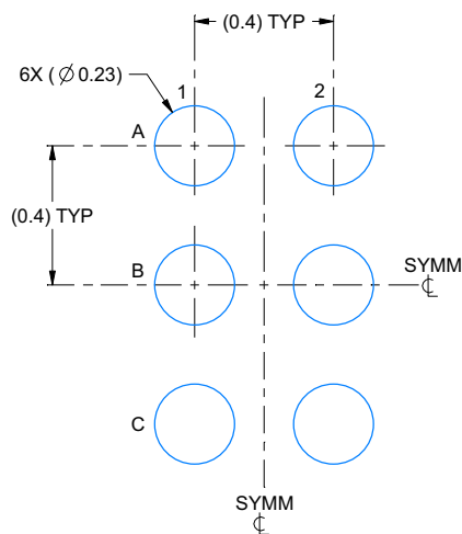
LAND PATTERN EXAMPLE SCALE:50X
