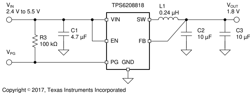
图 8-2. Typical Application of Fixed Output
