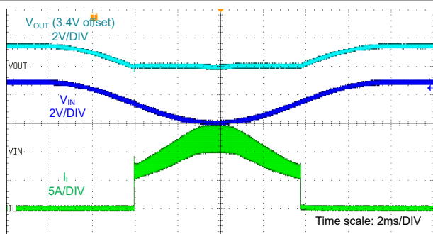
V_{OUT\_TAR} = 3.4V T_A = 25^\circ C 自动 PFM 负载 = 6A V_{IN} = 5V 至 2.2V 扫描
