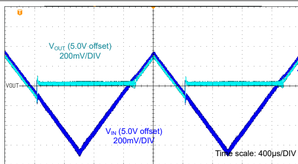
V_{OUT\_TAR} = 5.0V T_A = 25^\circ C 自动 PFM 负载 = 3A
