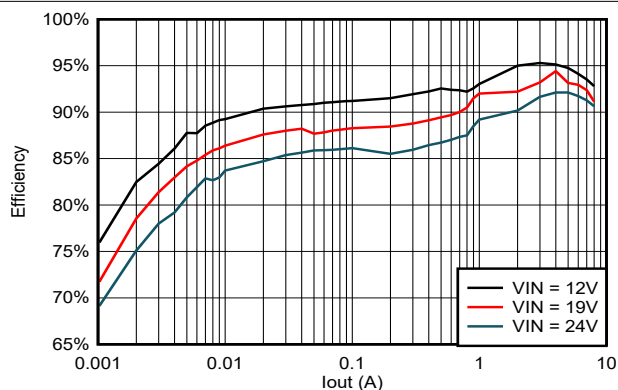
图 5-19. TPS56837 效率, V_{out} = 5V , F_{sw} = 1200kHz
