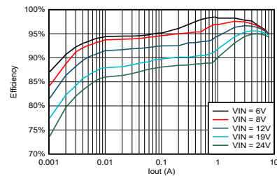
TPS56837 效率, Vout = 5V, Fsw = 500kHz
