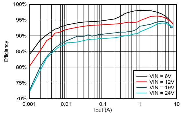
图 5-18. TPS56837 效率, V_{out} = 5V , F_{sw} = 800kHz
