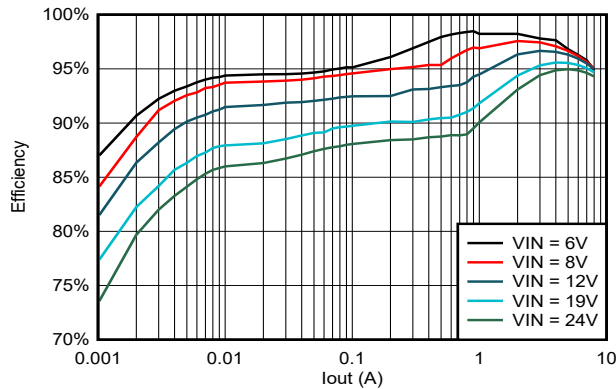
图 5-17. TPS56837 效率, V_{out} = 5V , F_{sw} = 500kHz
