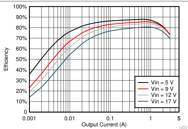
图 6-10. V_{OUT} = 1.05V 效率, L = 1.2\mu H
