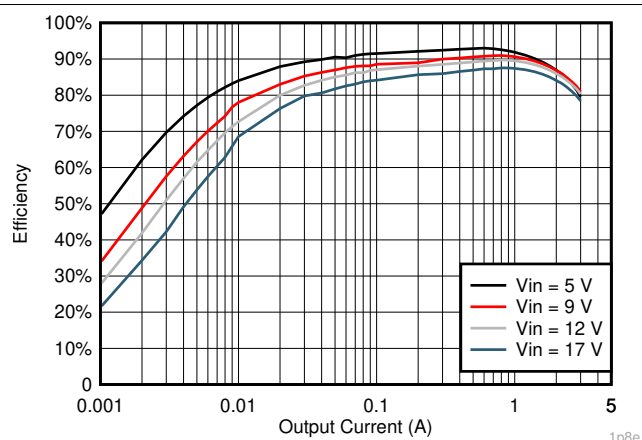
图 6-12. V_{OUT} = 1.8V 效率, L = 2.2\mu H
