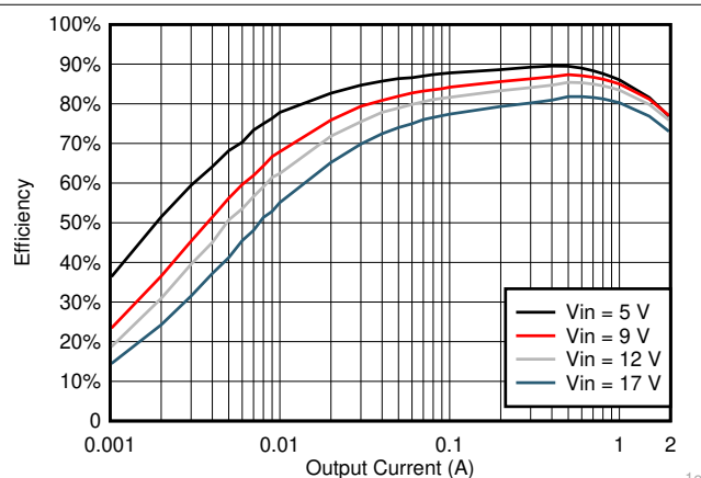
图 7-10. V_{OUT} = 1.05V 效率, L = 2.2\mu H
