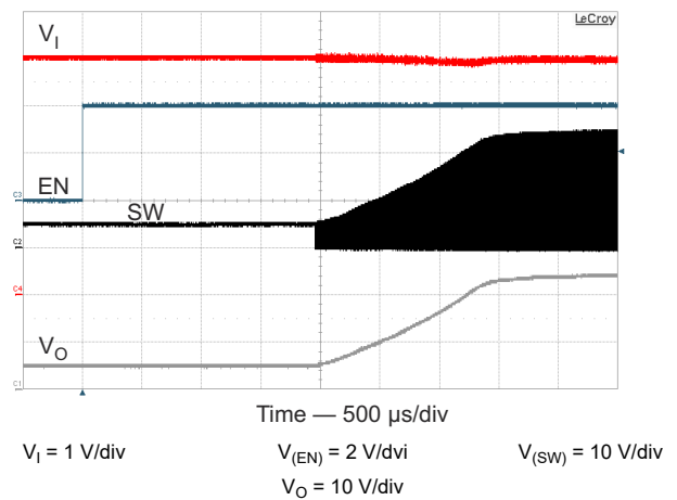
图 8-8. Start-Up
