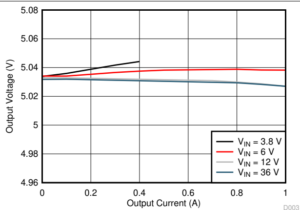
图 7-3. 5-V Output Regulation vs Load Current
