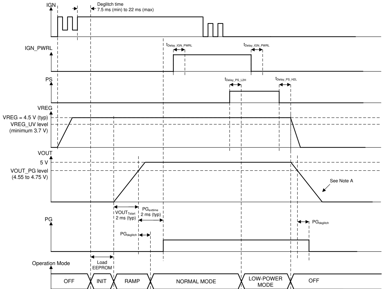
图 8-4. Power-Up and Power-Down Sequence With Low-Power Mode When IGN and IGN_PWRL are Low (Essentially When the ECU is in Sleep or Standby Mode)
