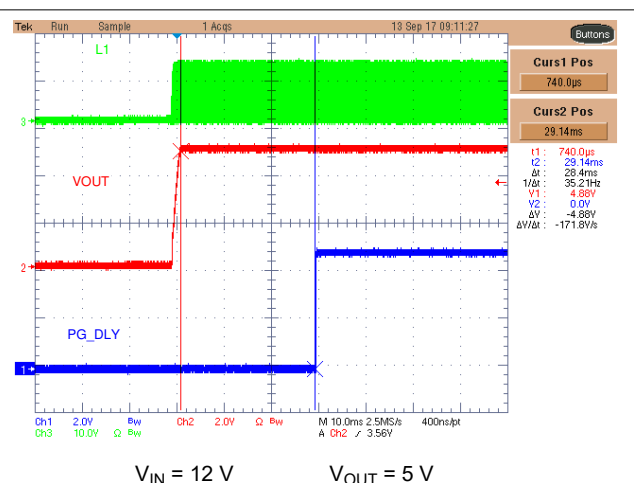
图 7-8. Power-Good Delay When PGDLY Connects to 100-kΩ Resistor
