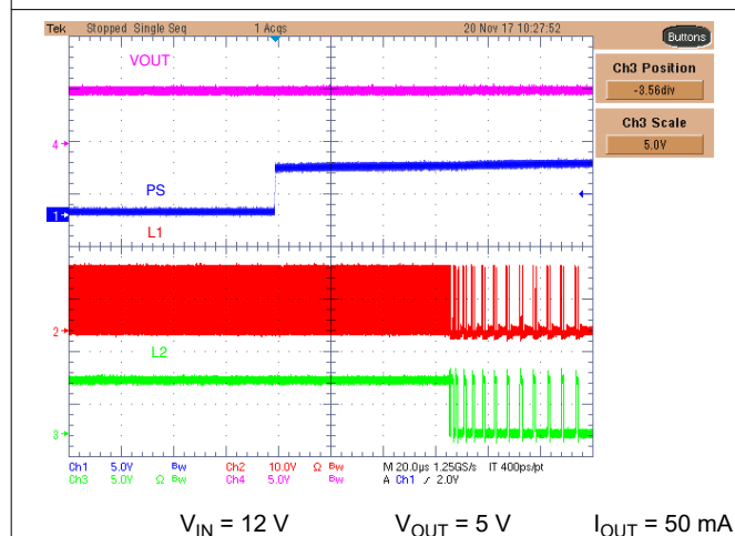
图 7-11. Low-Power Mode Enabling
