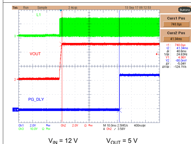
图 7-9. Power-Good Delay When PGDLY Connects to VREG
