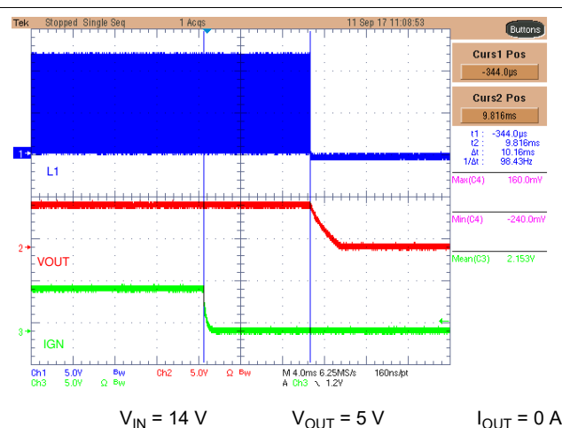
图 7-10. Ignition Shutdown Sequence
