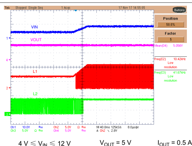
图 7-12. Step-Up to Step-Down Mode Transition
