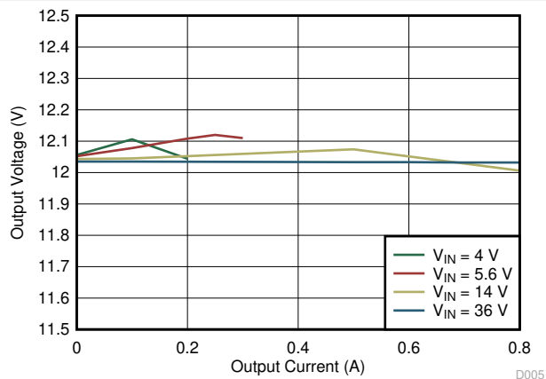
图 7-5. 12-V Output Regulation vs Load Current
