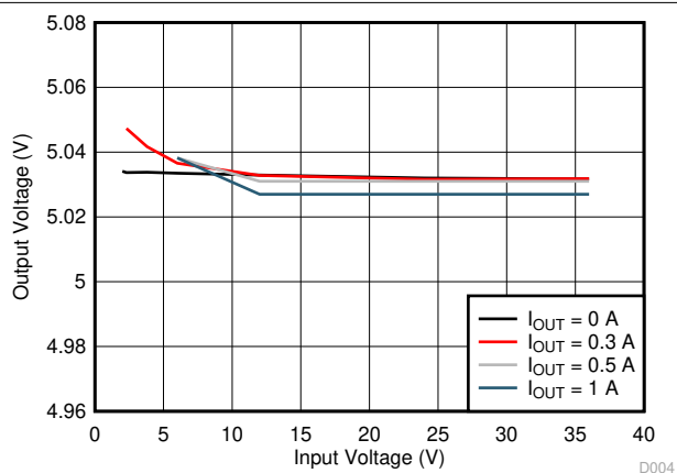
图 7-4. 5-V Output Regulation vs Input Voltage
