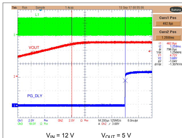
图 7-7. Power-Good Delay When PGDLY Is Grounded
