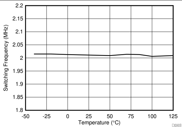
图 7-2. Switching Frequency vs Temperature
