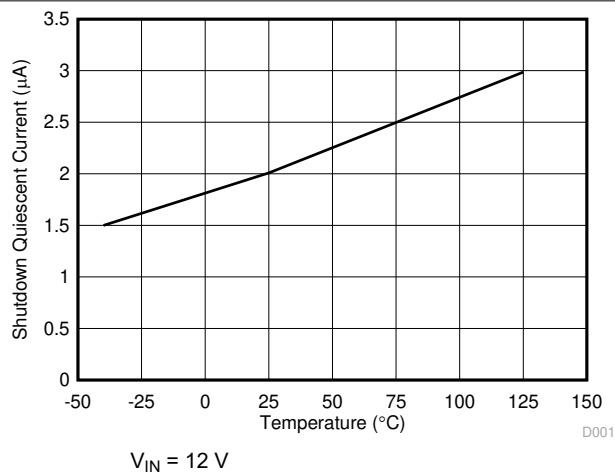
图 7-1. Shutdown I_Q vs Temperature
