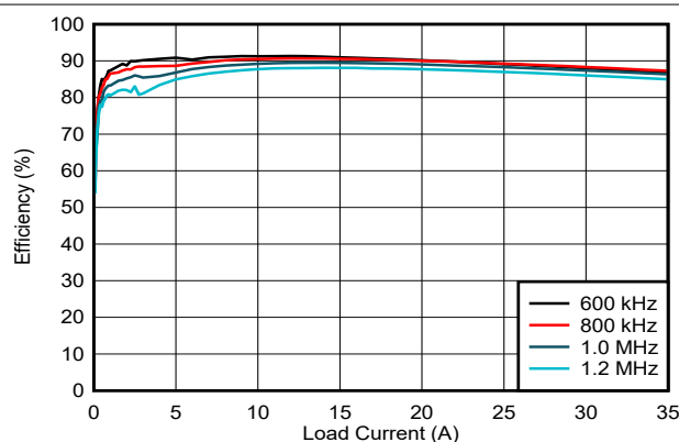
图 8-6. Efficiency, DCM, External 5-V Bias
