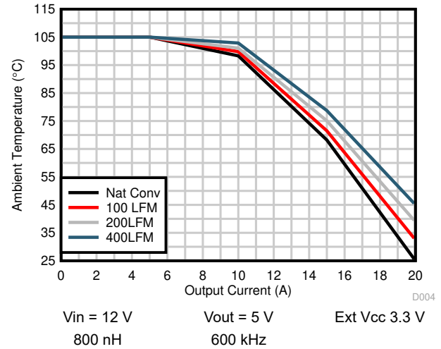
图 6-8. Safe Operating Area, V_{OUT} = 5\text{ V}
