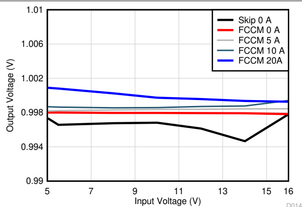
图 8-12. Output Voltage vs Input Voltage VCC = 3.3-V External Bias
