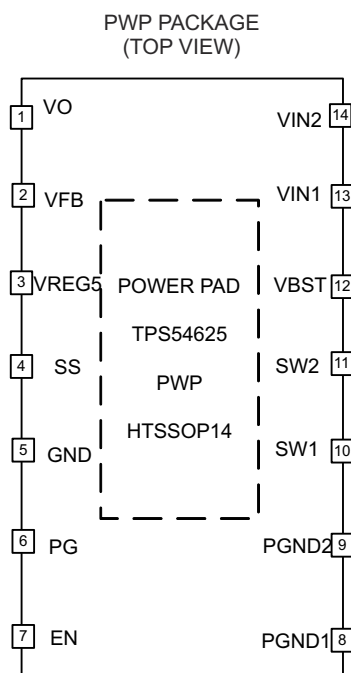
Pin Functions
