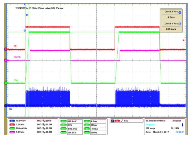
图 12. Output Voltage Start-Up and Shutdown
