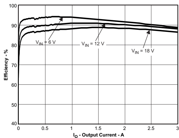
Figure 12. \text{VO1}=3.3\text{V} , Efficiency vs Output Current
