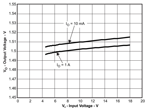
Figure 7. \text{VO2}=1.5\text{V} Output Voltage vs Input Voltage
