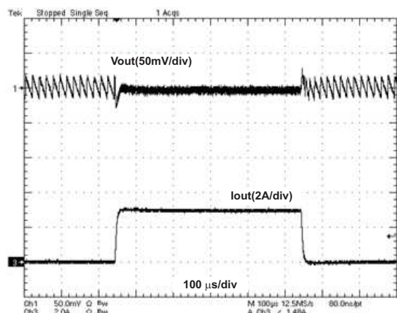
Figure 9. \text{VO2}=1.5\text{V} , 0A to 3A Load Transient Response
