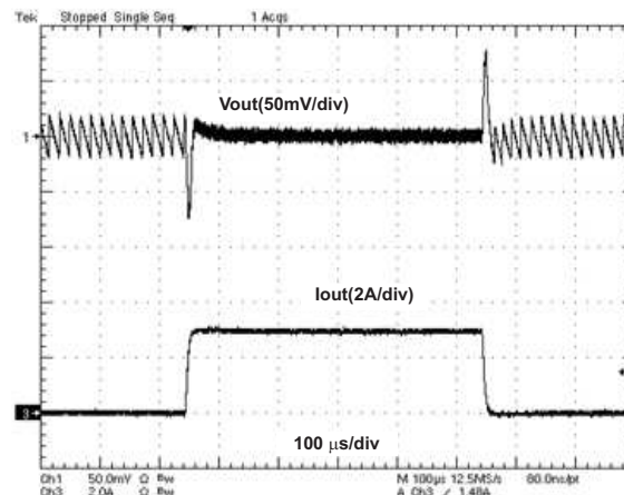
Figure 8. \text{VO1}=3.3\text{V} , 0A to 3A Load Transient Response
