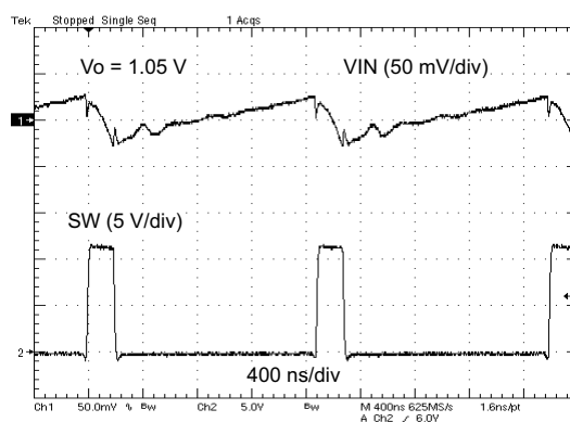
Figure 15. VOLTAGE RIPPLE AT INPUT ( I_O = 3\text{ A} )
