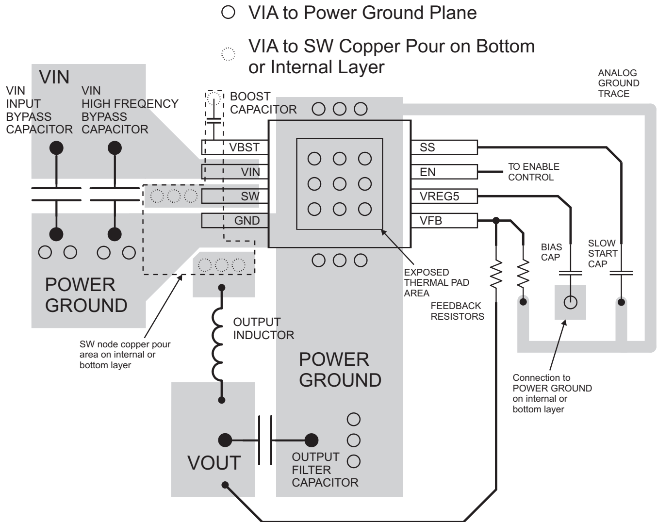
Figure 17. PCB Layout
