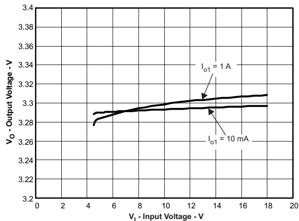
Figure 6. V_{O1}=3.3\text{V} Output Voltage vs Input Voltage
